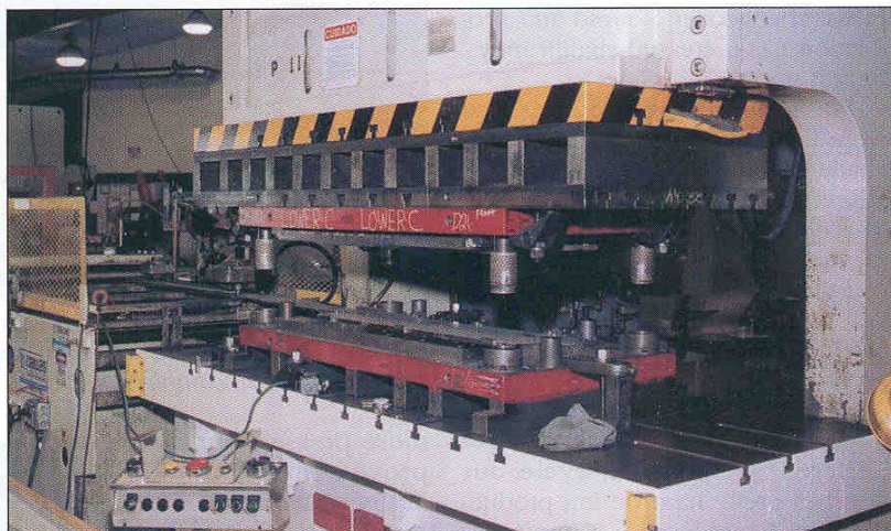
An example of a single-stroking operation where the blank is cut to length and its corners are trimmed. Then the blank is manually moved forward through two additional stations to complete the part.
