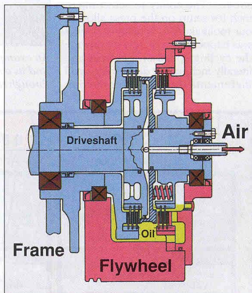
Fig.2—The wet clutch allows for high single-stroking rates when a press is used in hand-fed operations or with automation. A hardened and ground main drive gear and pinion—which reduce backlash and maintenance while extending gear life—are standard features on Aida-DTC gap presses.
